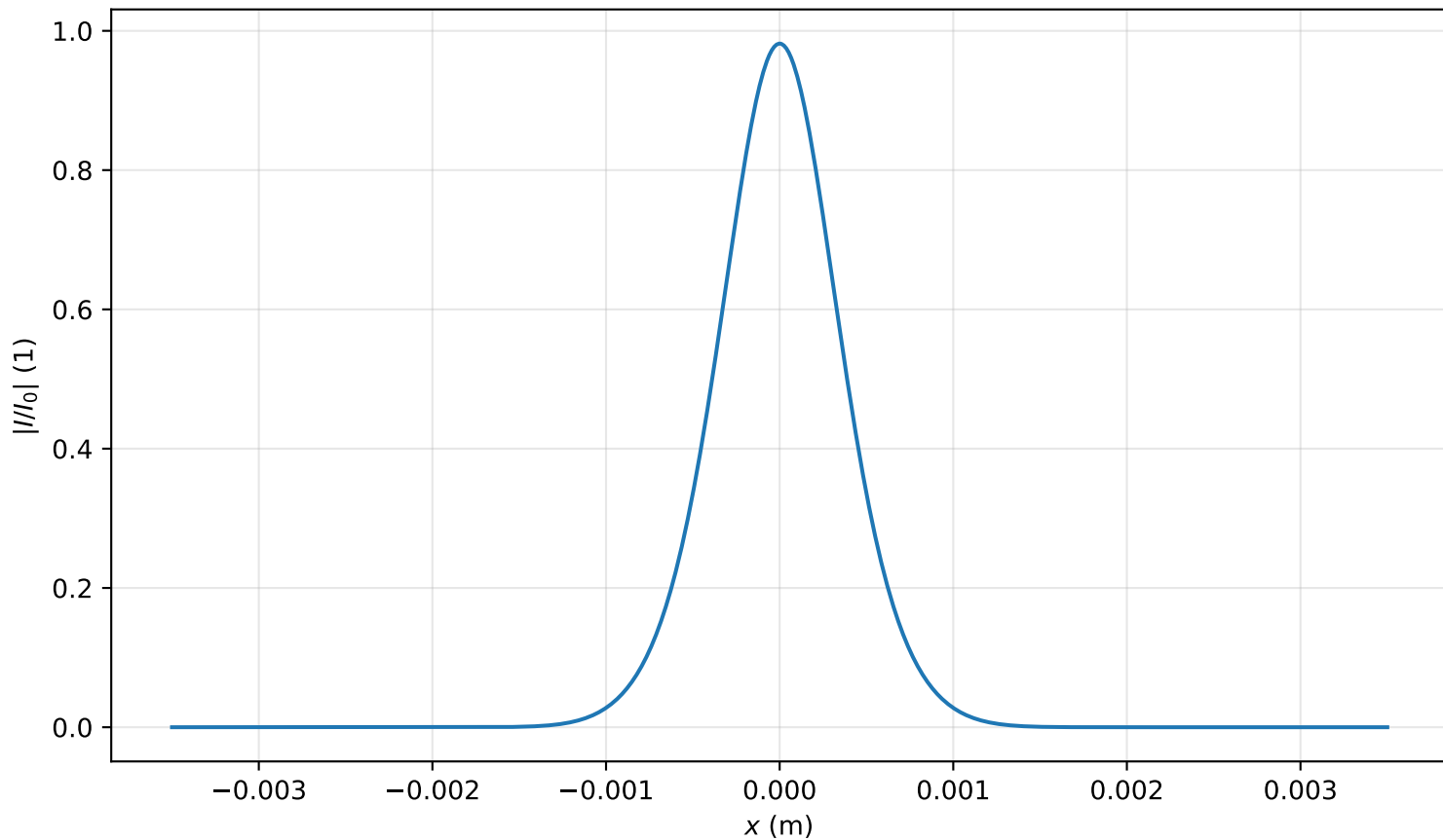
Intensity profile I(x, y = 0, z = 1.035m)/I_0 , P_{in}=0.4P_{cr} , artificial time
